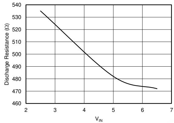
Figure 6-8. Discharge Resistance vs V_{IN}
