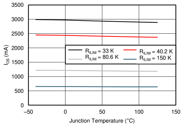
Figure 6-7. I_{OS} vs Junction Temperature
