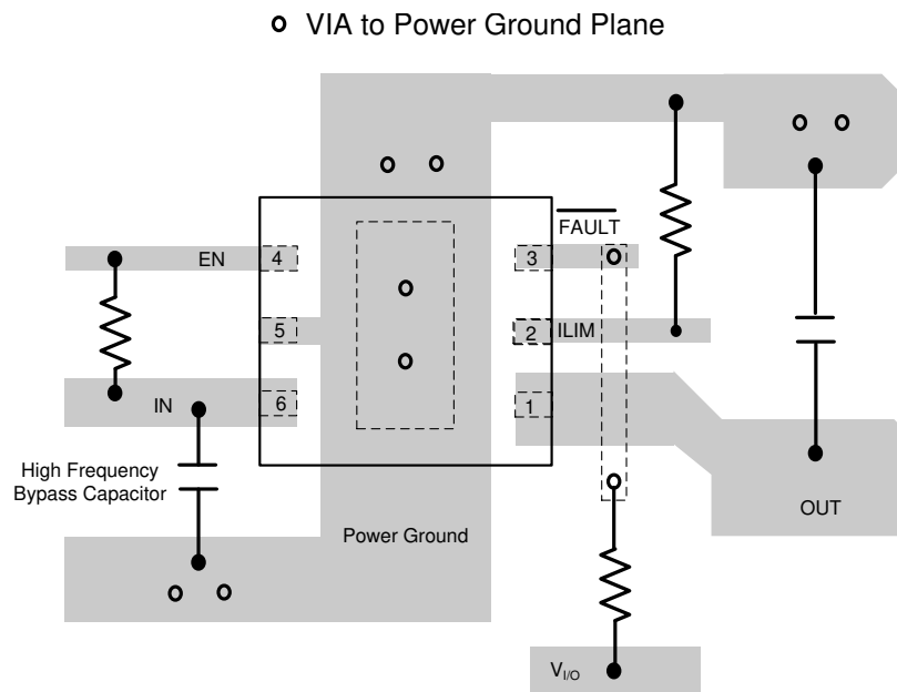
Figure 11-1. TPS25200 Board Layout
